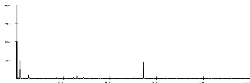
Figure 4. RRM cross-spectrum of Neuroigin2 proteins and \alpha - and \beta - Neuroxin2 proteins.
