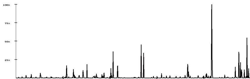
Figure 1. RRM cross-spectrum of Neuroigin3 proteins.
