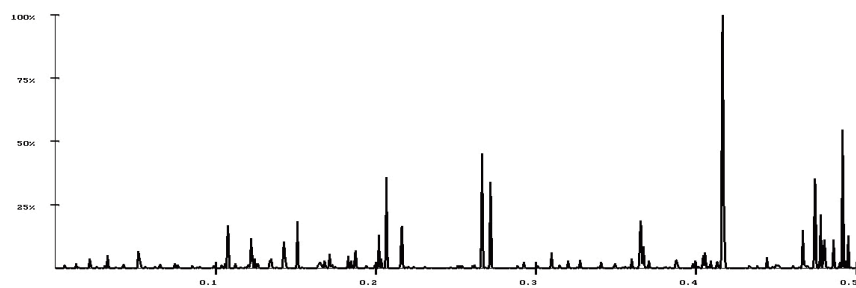
Figure 2. RRM cross-spectrum of Neuroigin3 proteins and \alpha -Neurexin3 proteins.
