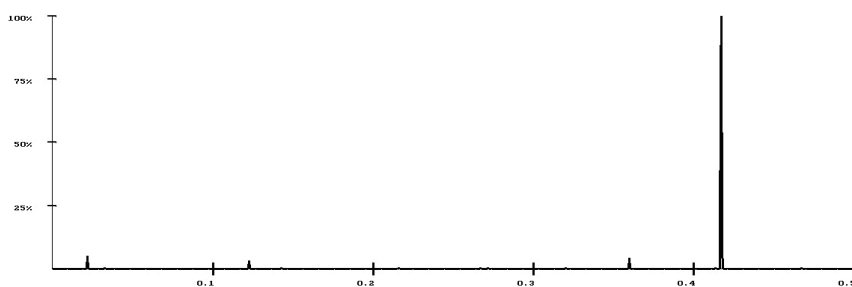
Figure 3. RRM cross-spectrum of Neuroigin proteins, including Neuroigin1, 3 and 4.
